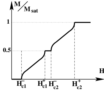
Figure 2. Schematic drawing of the magnetization (in units of saturated magnetization M_{\text{sat}} ) of a two-leg isotropic ladder with alternating rungs as a function of the external magnetic field.
